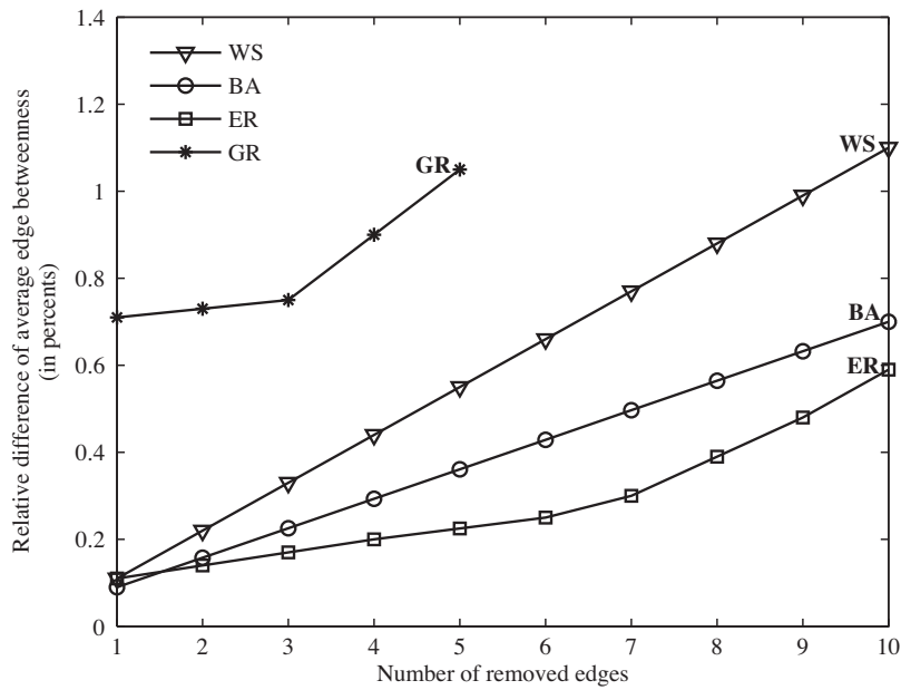
Fig. 3. Relative difference of the average edge betweenness after a finite number of edges are removed (using edge betweenness).
