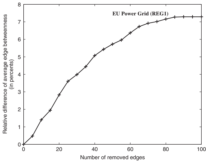
Fig. 7. Relative difference of the b_{nor} after some of the edges are removed (using edge betweenness) for the region 1 of the EU power grid.
