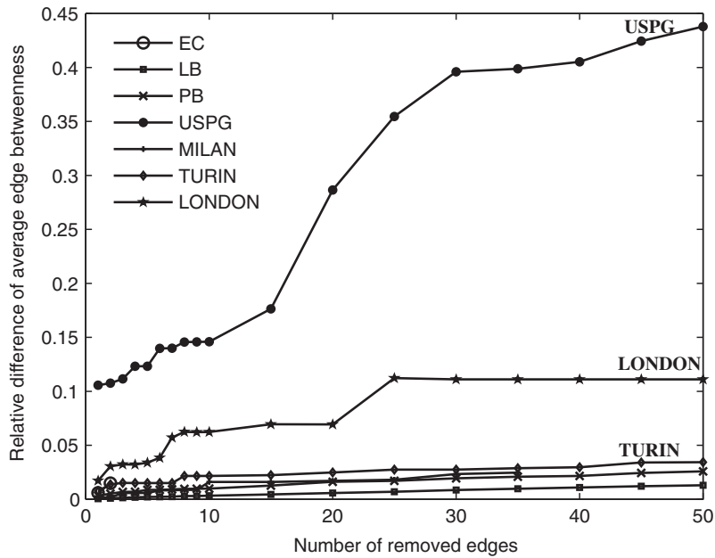
Fig. 6. Relative difference of the b_{nor} after some of the edges are removed (using edge betweenness).
