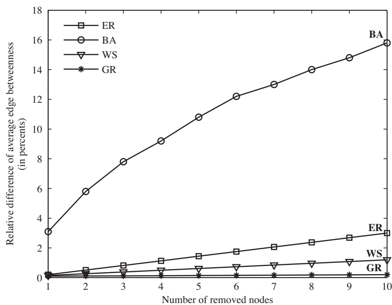
Fig. 2. Relative difference of the average edge betweenness after a finite number of nodes are removed (using PageRank).
