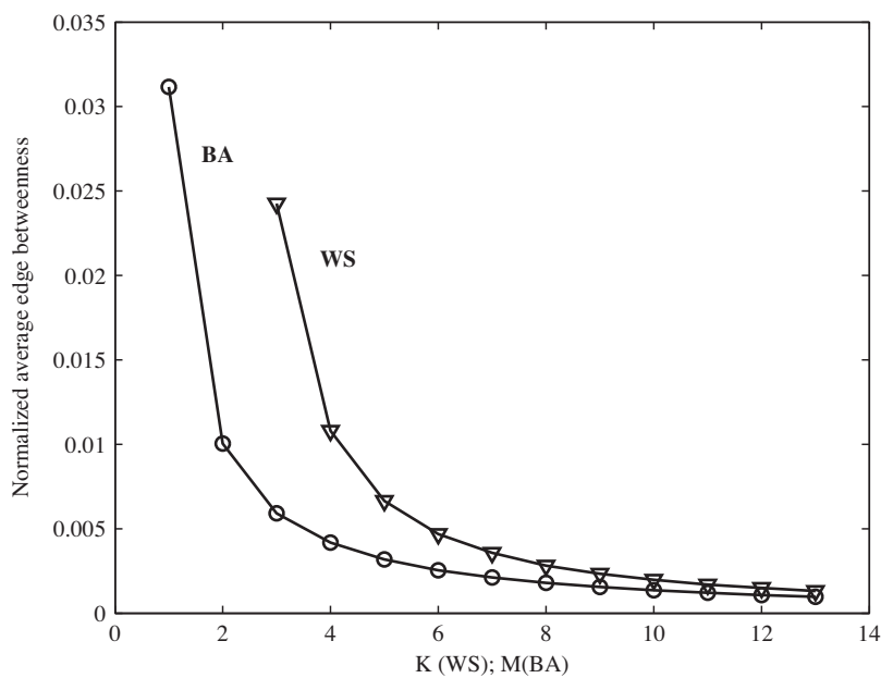
Fig. 4. Normalized average edge betweenness WS and BA networks versus K and M.
