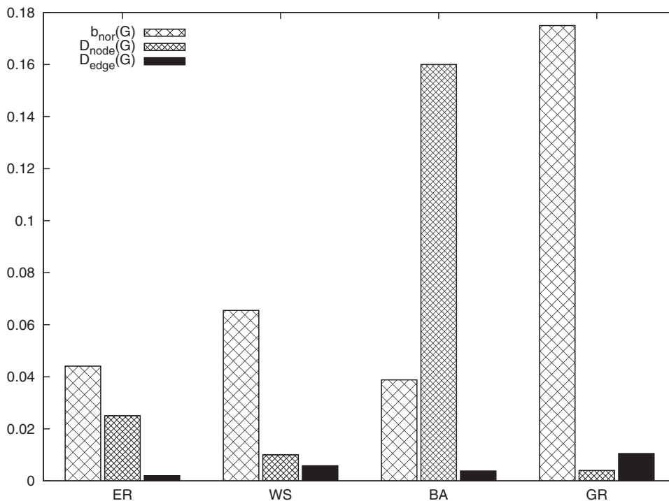
Fig. 1. Dynamical robustness of synthetic networks.
