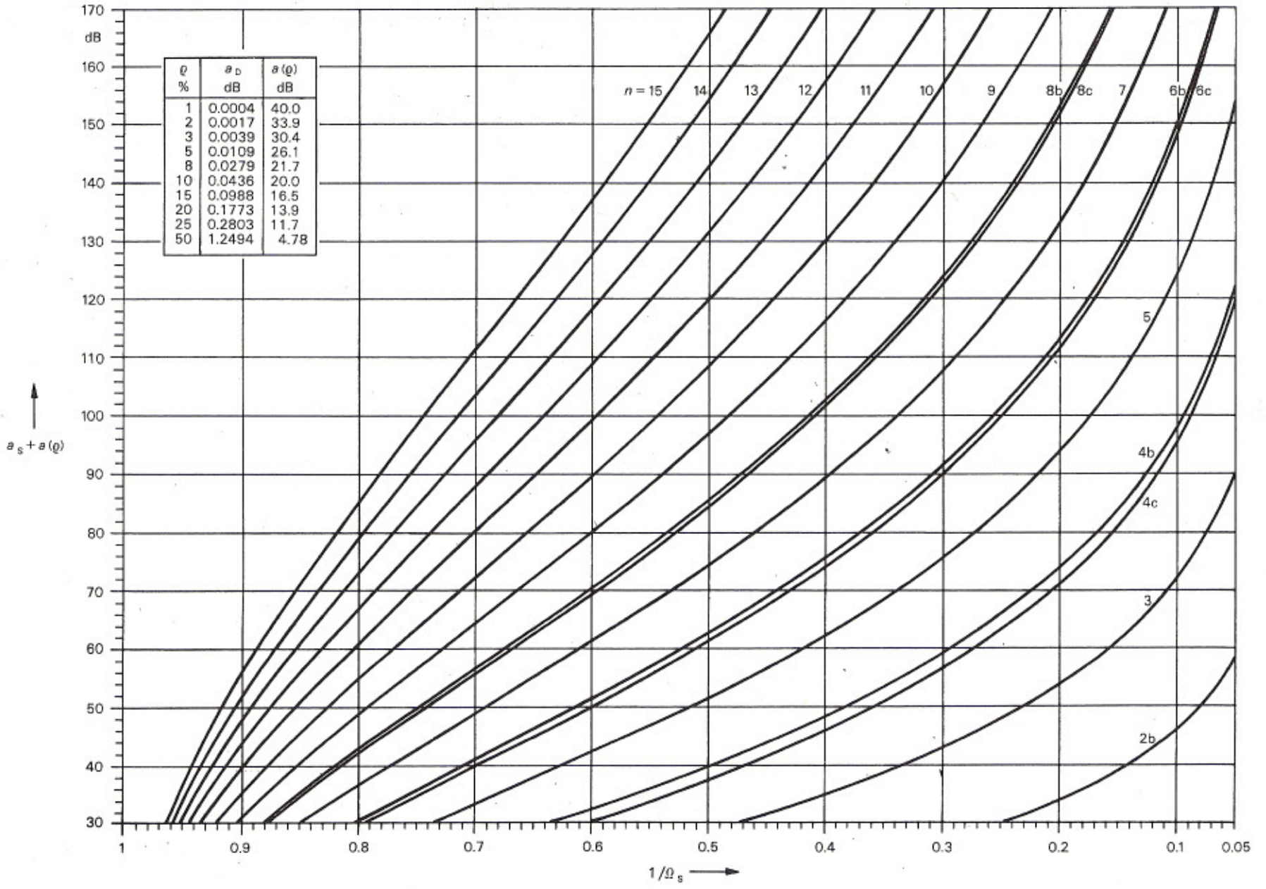
Fig. 2.6 Diagram to estimate the degree of Chebyshev lowpass filters
